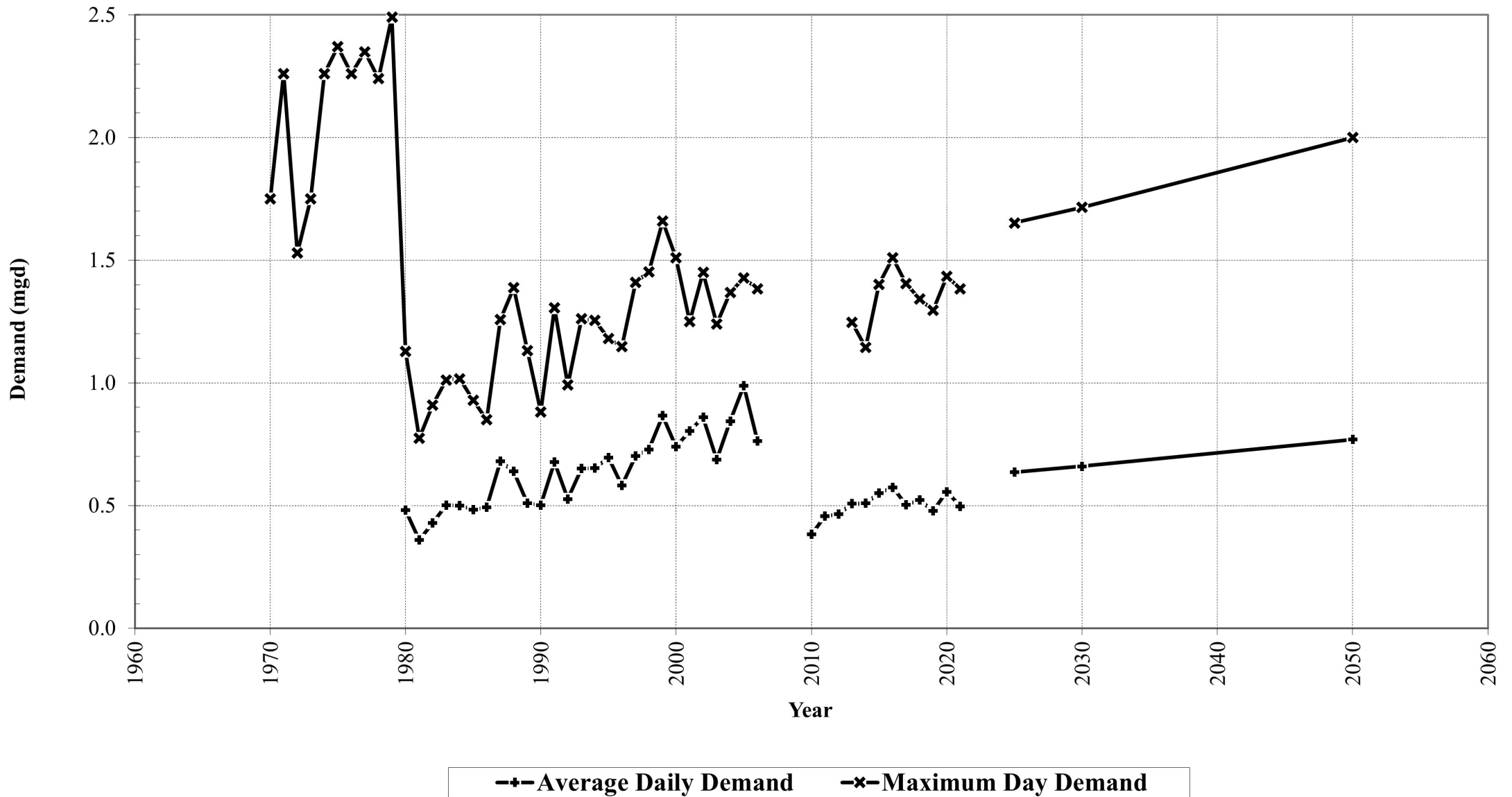
Figure 1. Historic Water Use, Barnstable Fire District, MA
